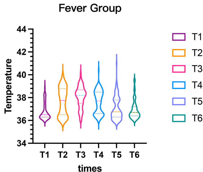
FIGURE 1. Violin plot of temperature descriptive of fever group.
