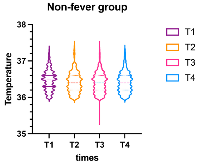
FIGURE 2. Violin plot of temperature descriptive of the non-fever group.
