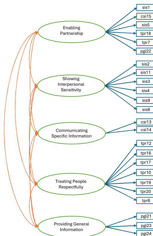
FIGURE 3. Five-factor model.
