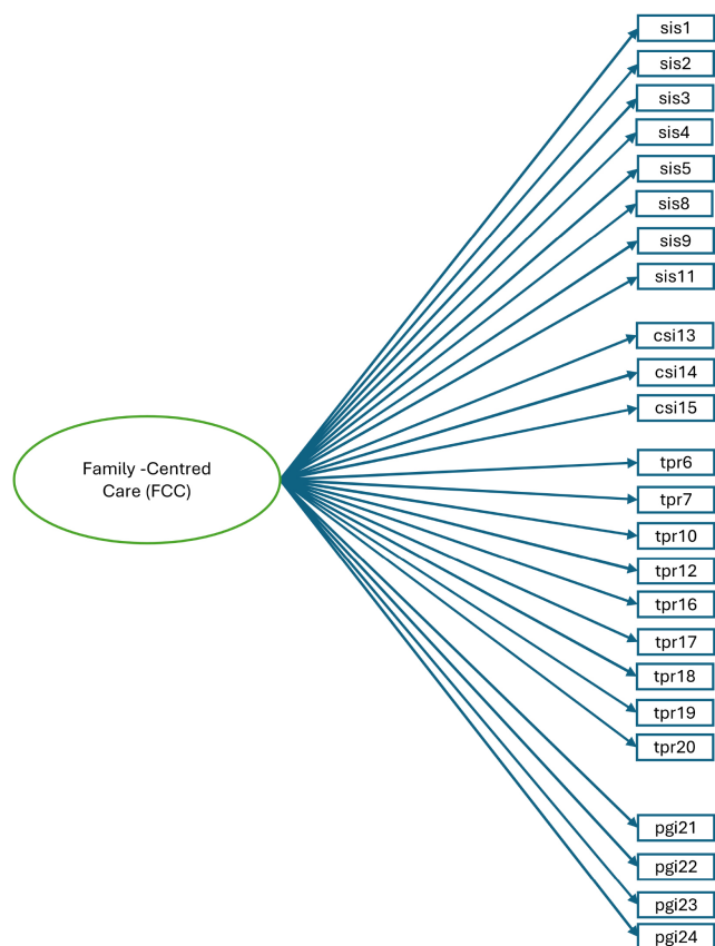
FIGURE 1. Unidimensional model.
